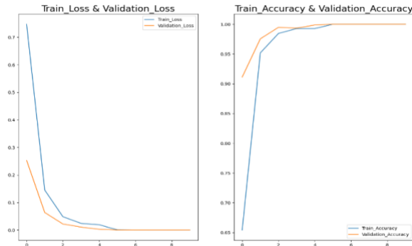
Fig. 3. Training Curves
