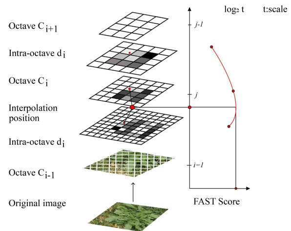
Fig. 4: Scale pyramid space with n number of octaves and n number of intra-octaves for keypoints detection at i represents the level
